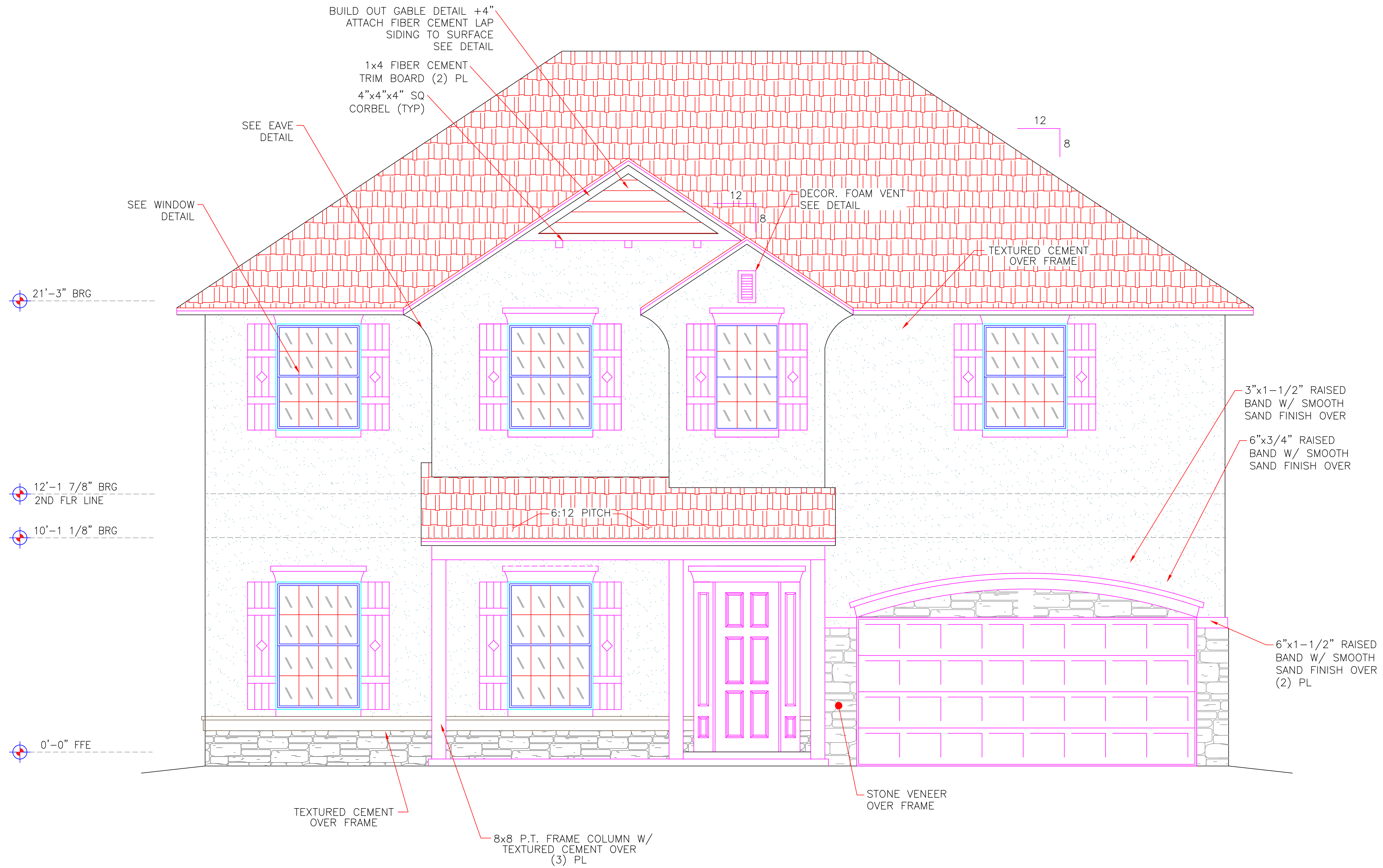
FRONT ELEVATION SCALE: 1/4" = 1'-0"
