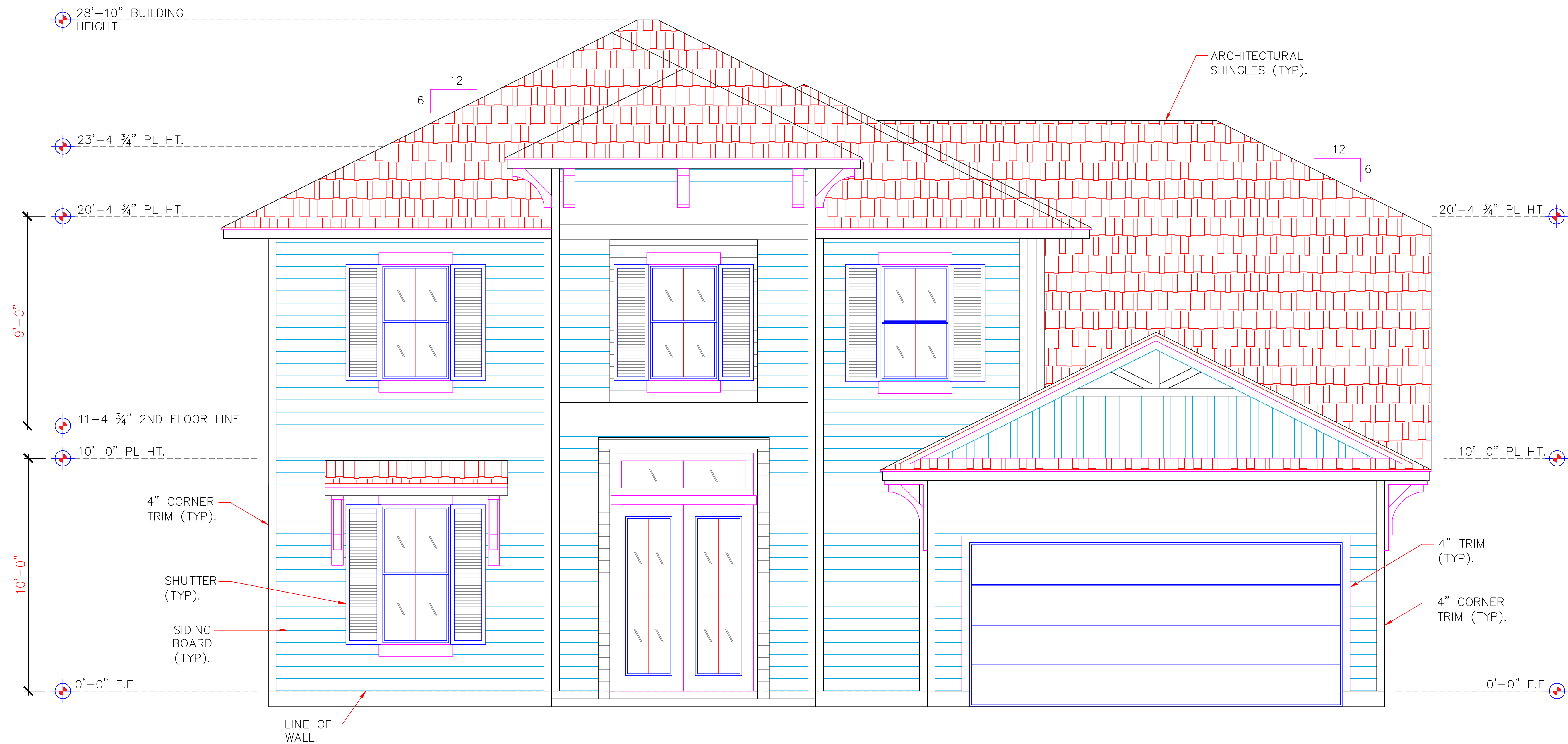
FRONT ELEVATION SCALE: 1/4" = 1'-0"
